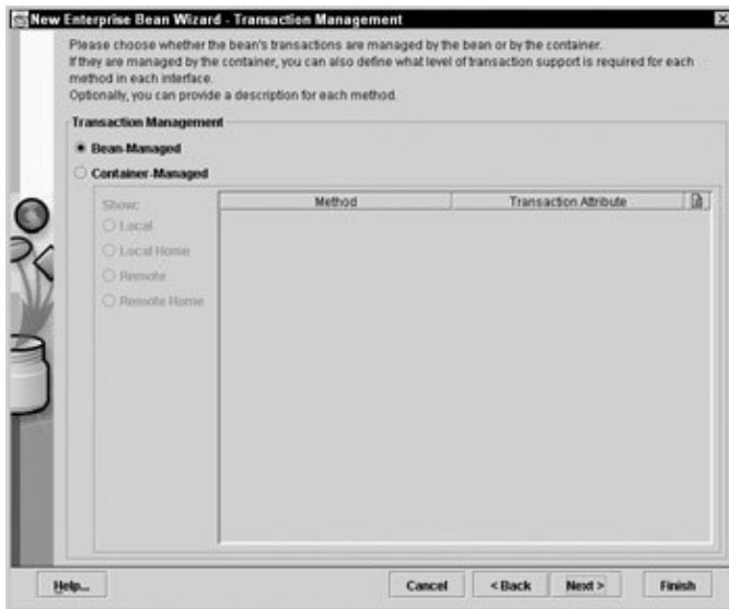
Figure A–8: Selecting transaction attributes for the methods of your EJB
