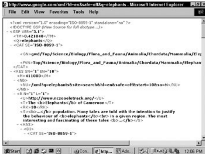
Figure 10–2: The Google elephant search in XML
